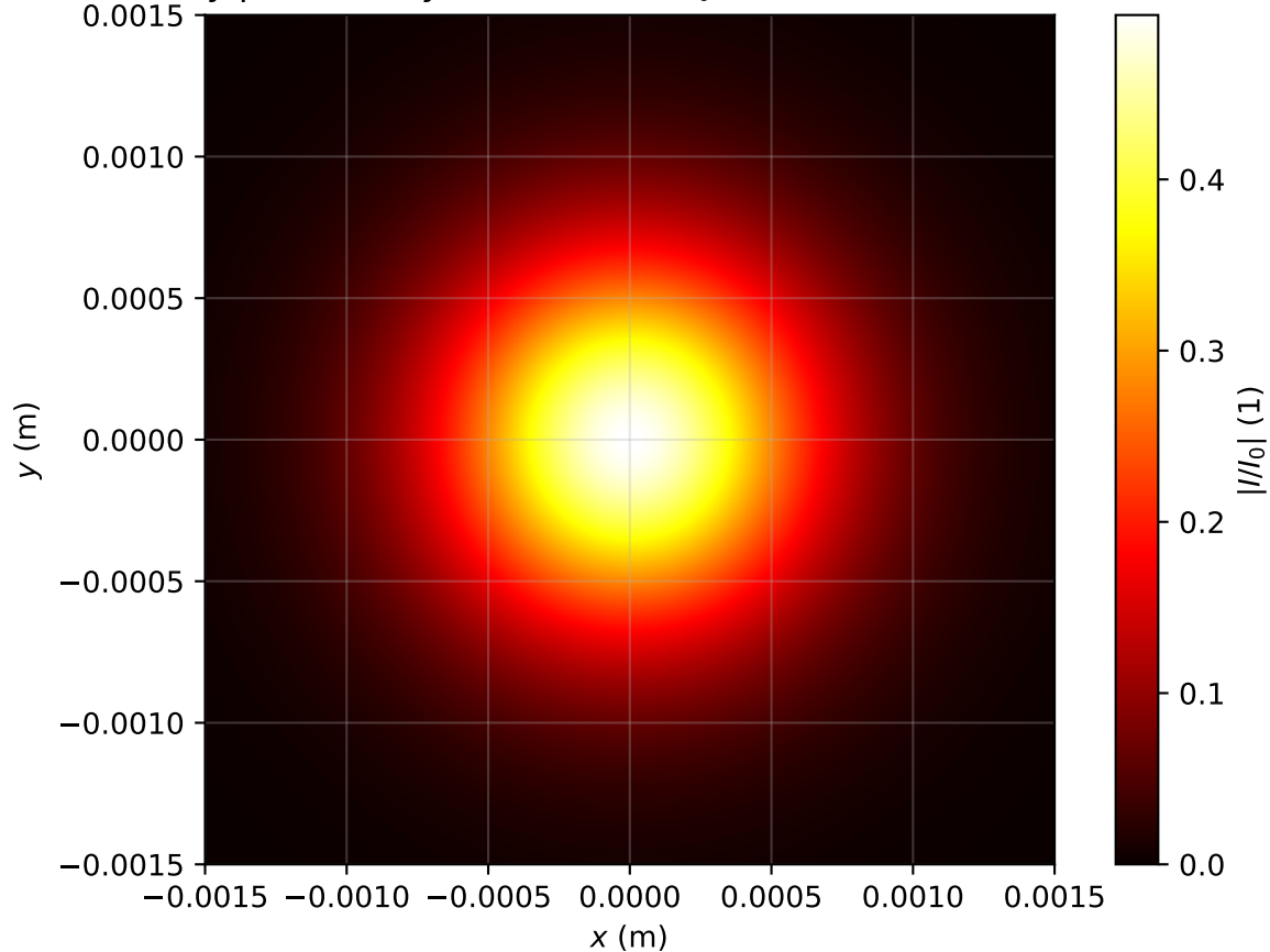
Intensity profile I(x, y, z = 3.344m)/I_0 , \text{Pin}=0.5\text{Pcr} , artificial time
